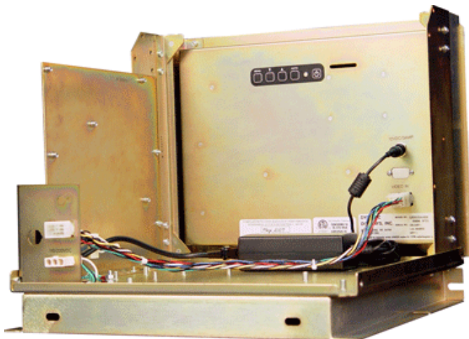
Rear View of a 14.1" LCD Open Frame Monitor Mounted on 14" CRT Chassis. Existing CRT Chassis Not Provided
